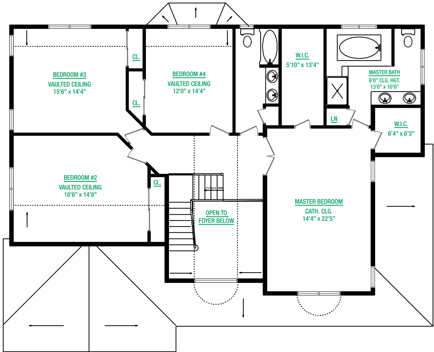
SECOND FLOOR PLAN LIVING AREA = 1628 SQ.FT.
